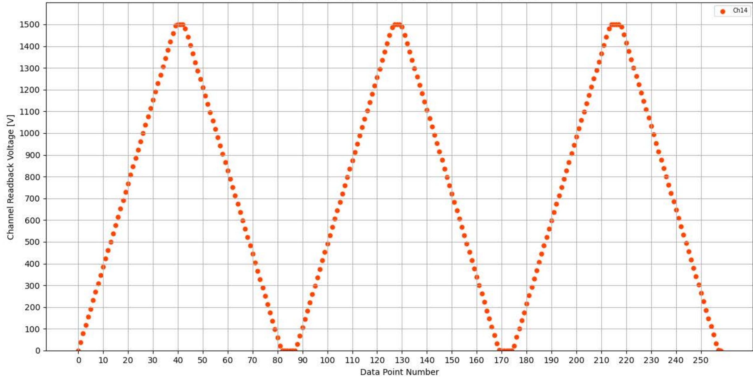
Voltage Ramp Test (Python) Bd #356, Slot #14, Ch #14
