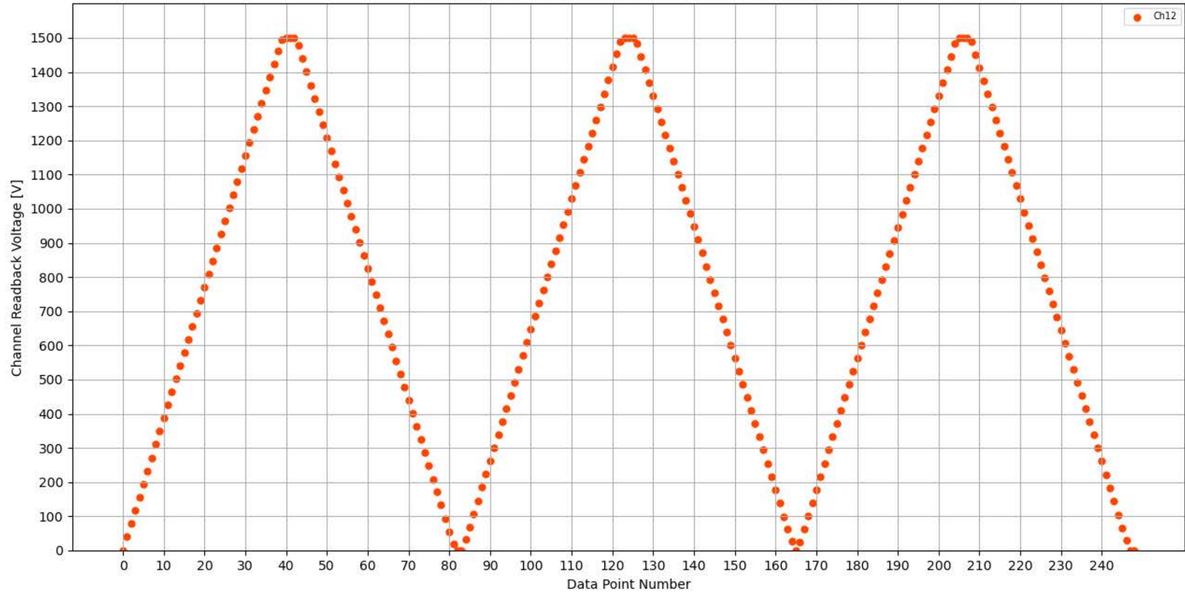
Voltage Ramp Test (Python) Bd #356, Slot #14, Ch #12
