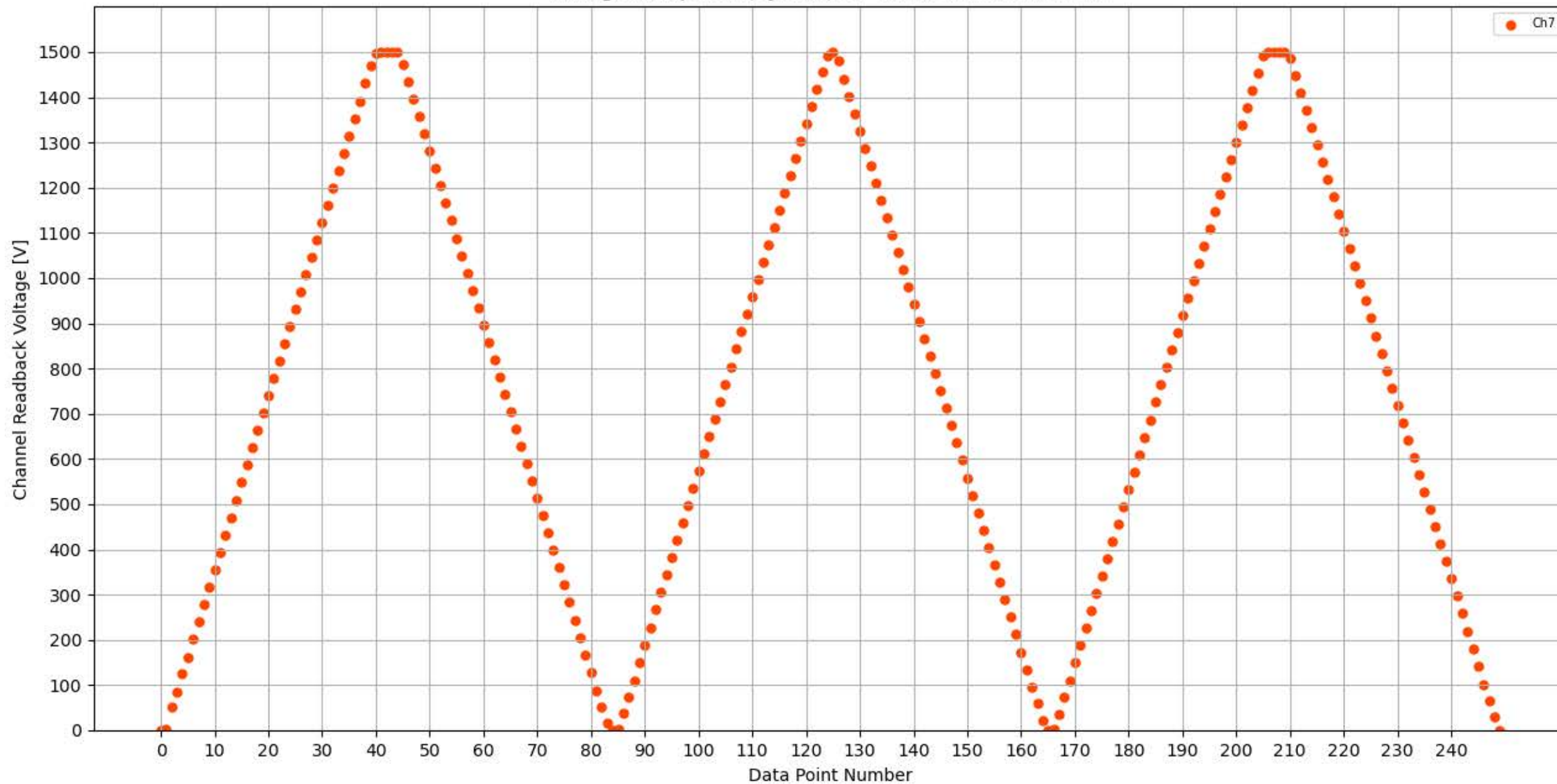
Voltage Ramp Test (Python) Bd #356, Slot #14, Ch #7
