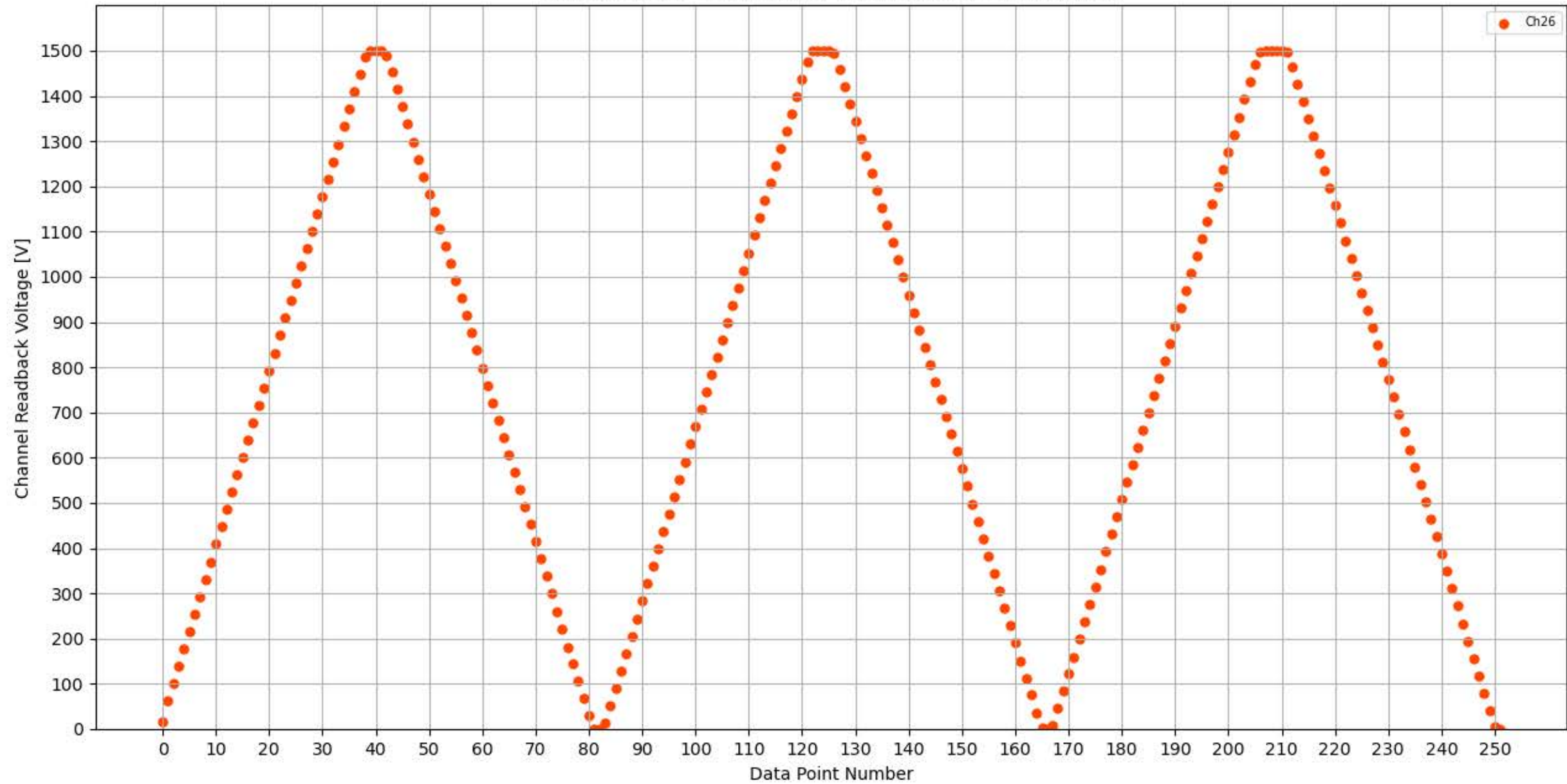
Voltage Ramp Test (Python) Bd #356, Slot #14, Ch #26
