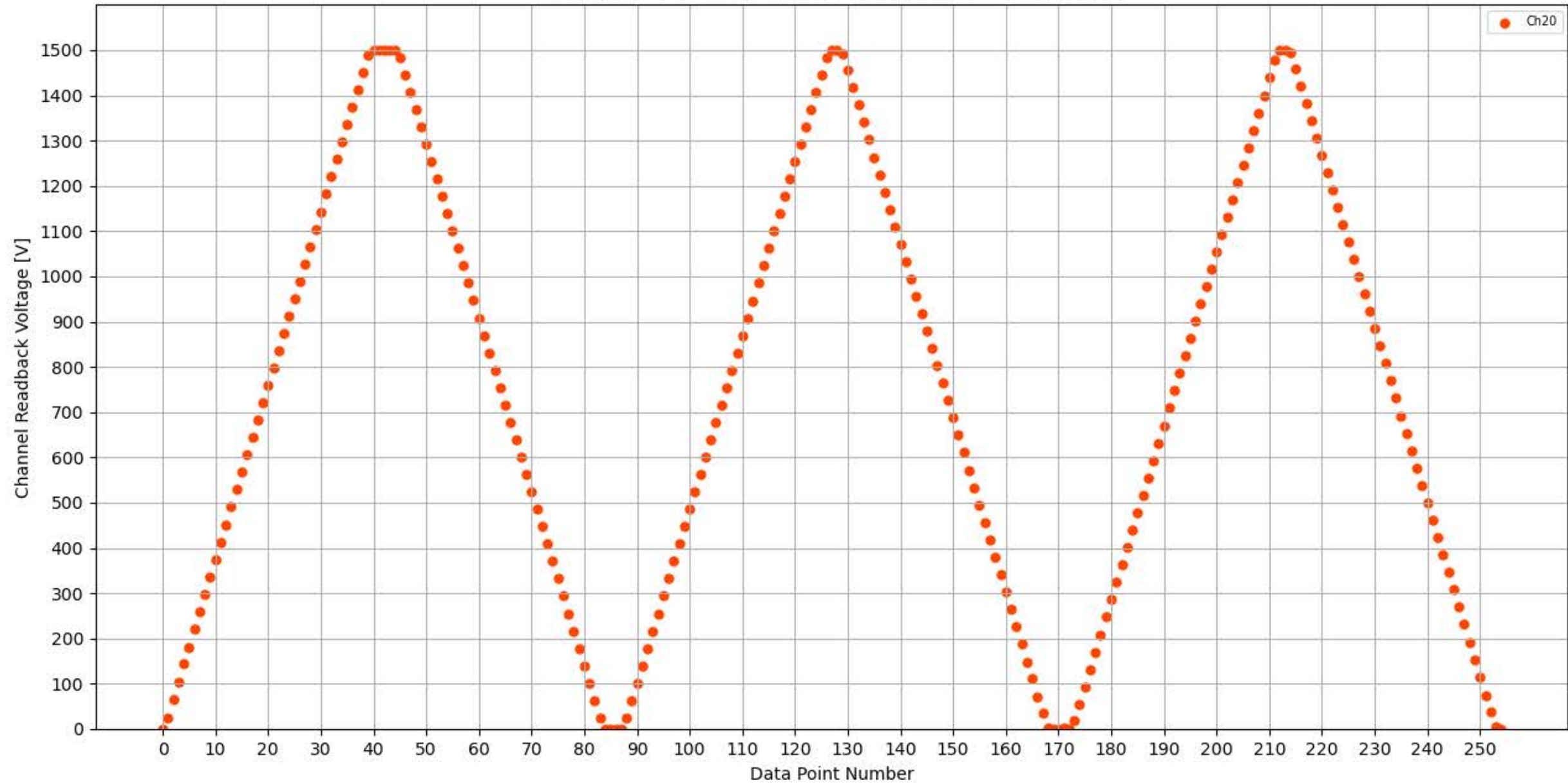
Voltage Ramp Test (Python) Bd #356, Slot #14, Ch #20
