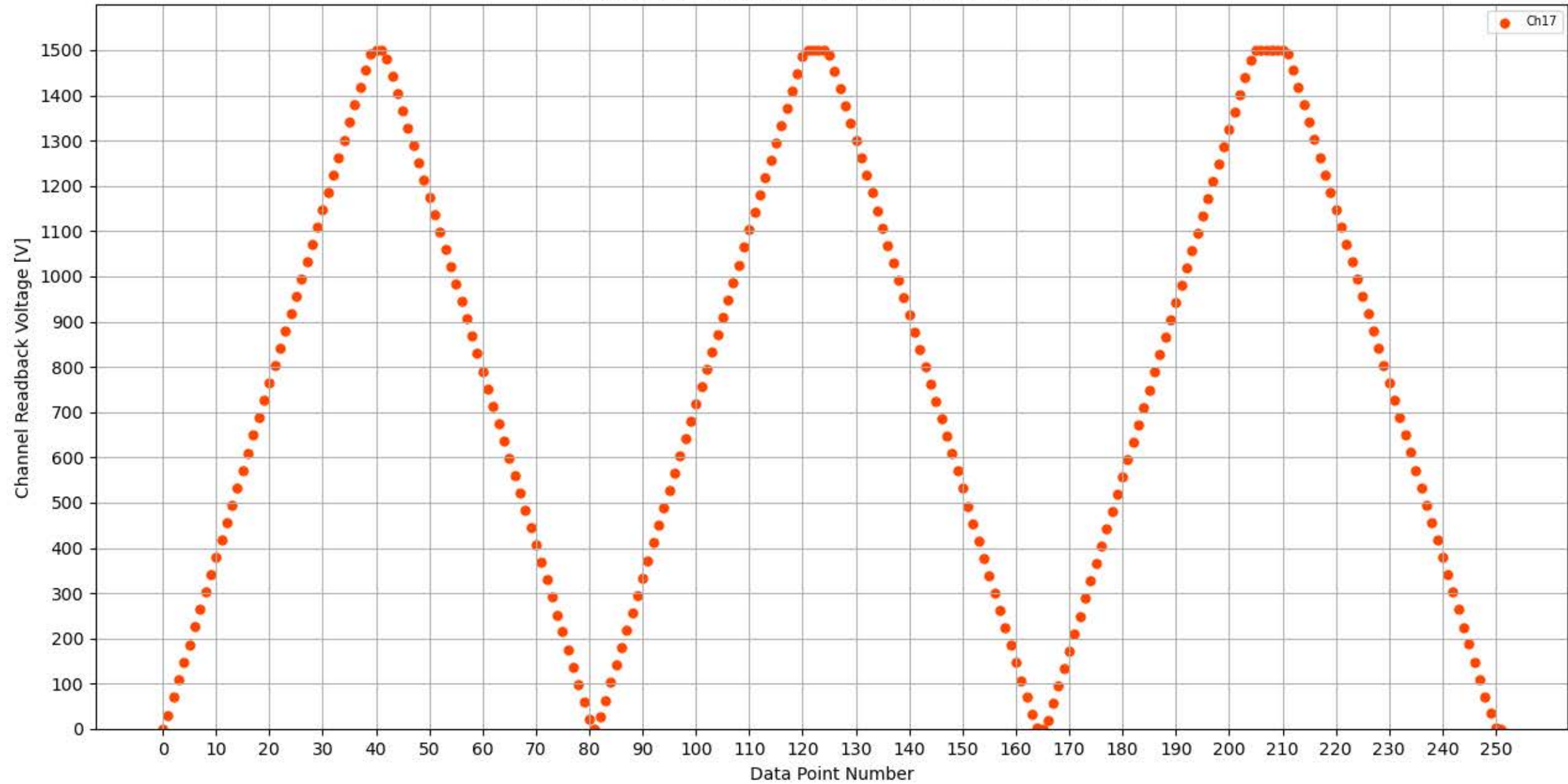
Voltage Ramp Test (Python) Bd #356, Slot #14, Ch #17
