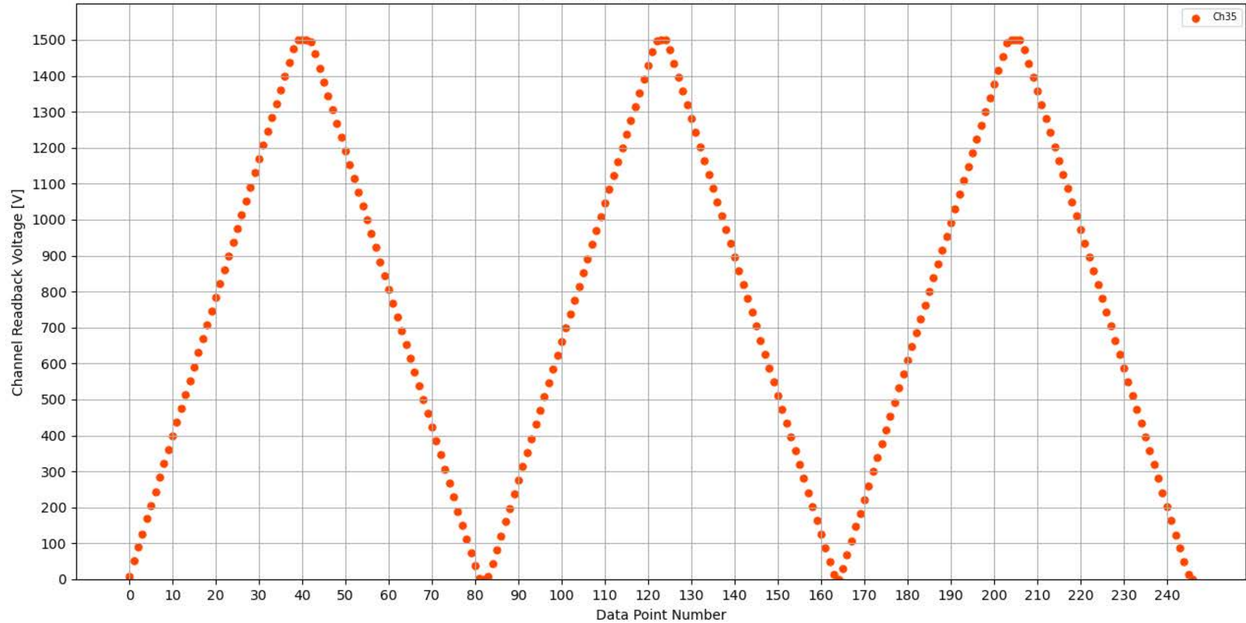
Voltage Ramp Test (Python) Bd #356, Slot #14, Ch #35
