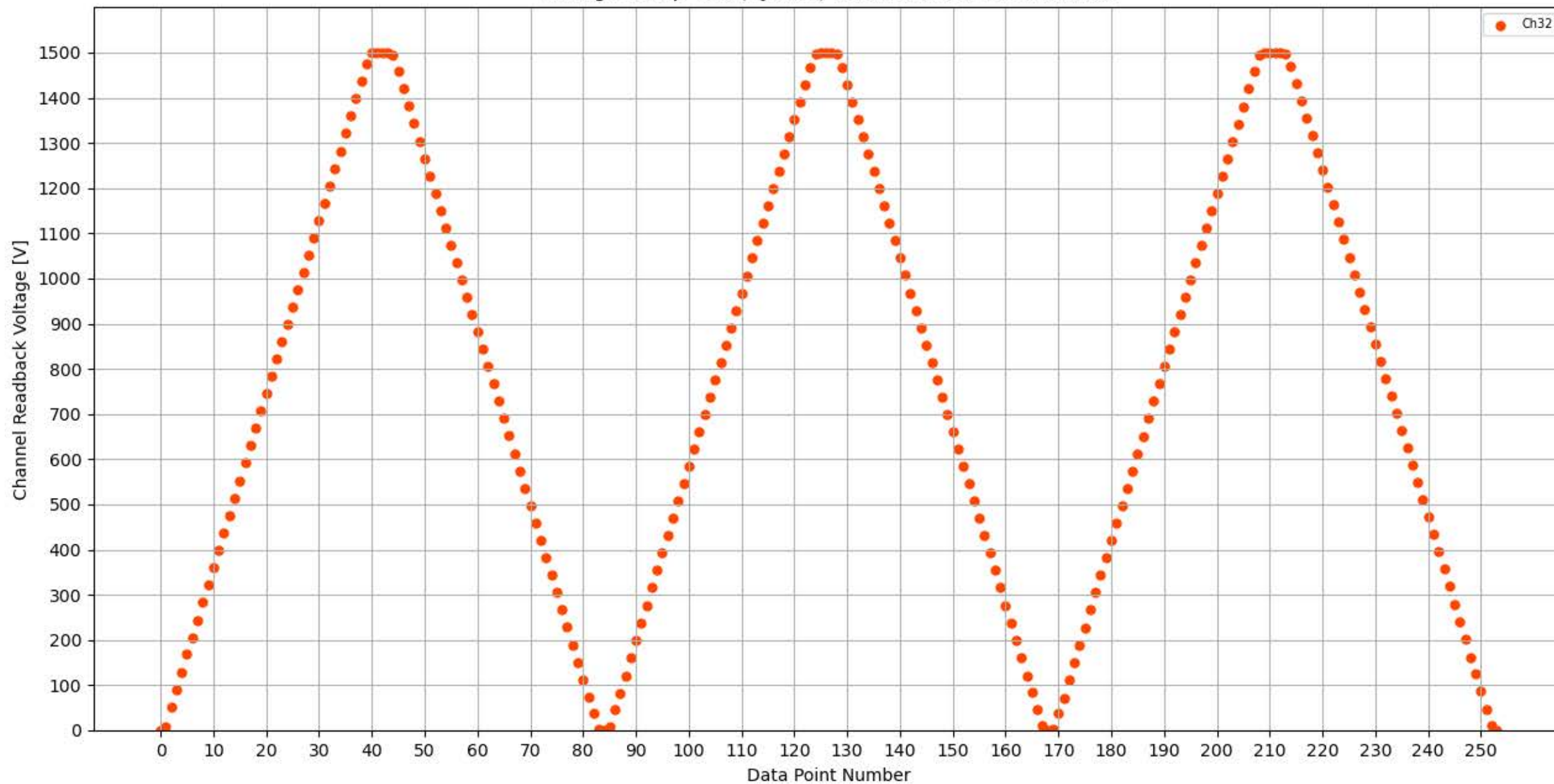
Voltage Ramp Test (Python) Bd #356, Slot #14, Ch #32
