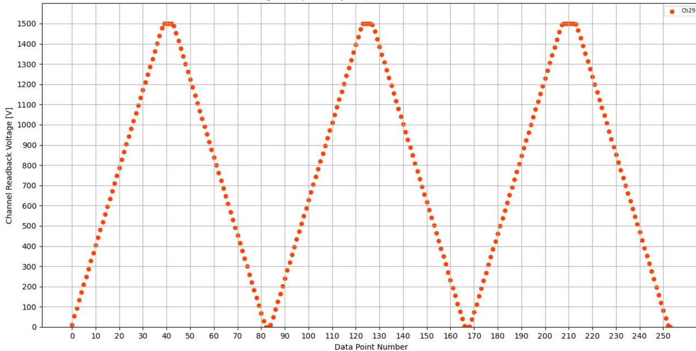
Voltage Ramp Test (Python) Bd #356, Slot #14, Ch #29
