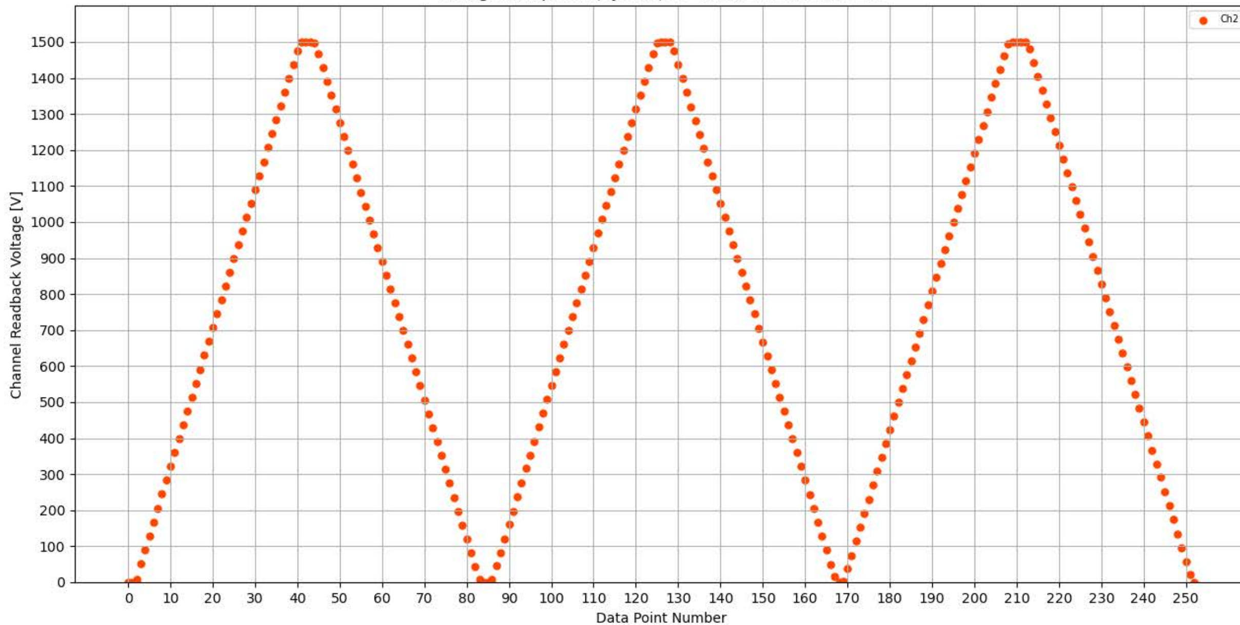
Voltage Ramp Test (Python) Bd #356, Slot #14, Ch #2
