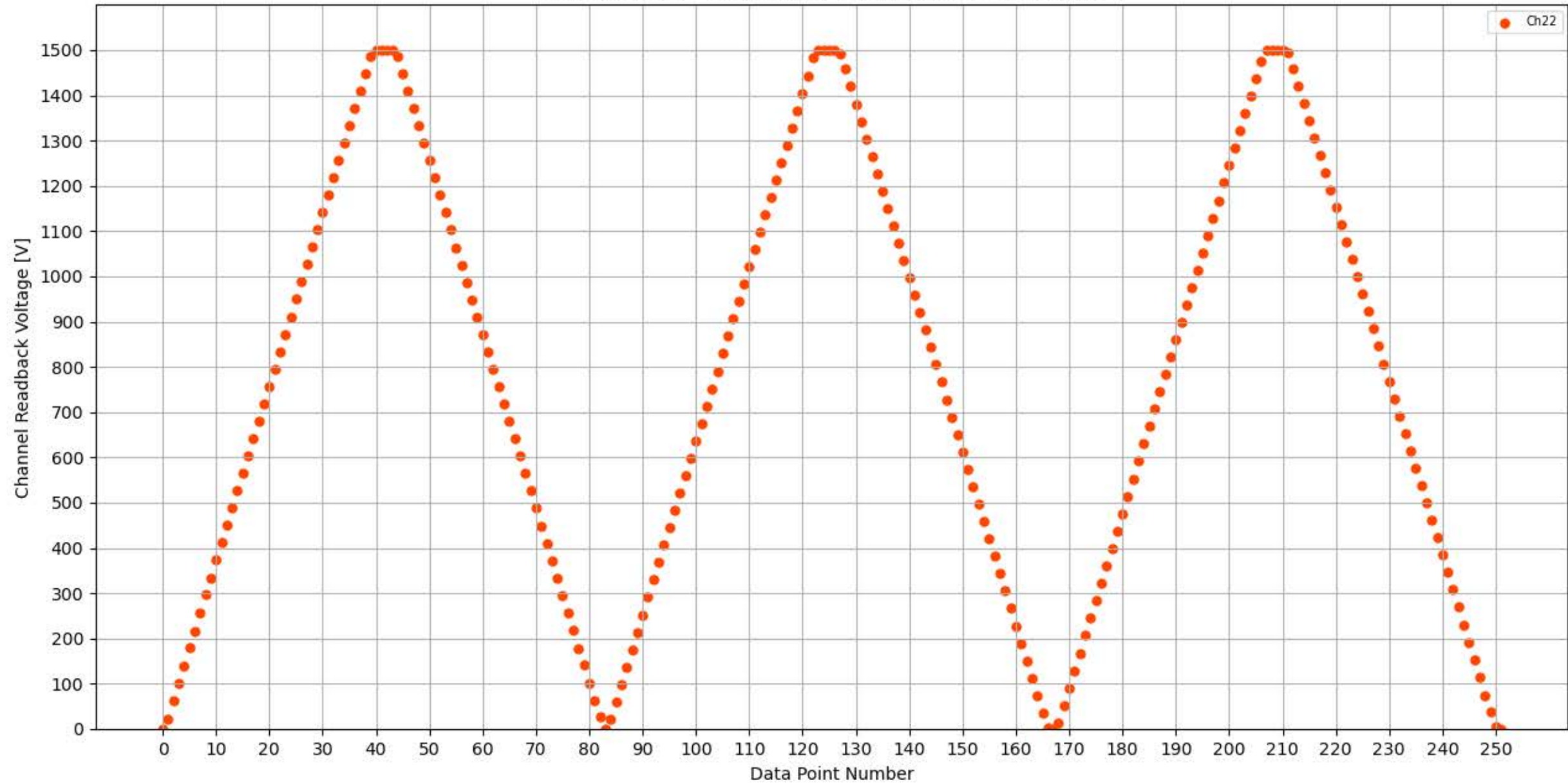
Voltage Ramp Test (Python) Bd #356, Slot #14, Ch #22
