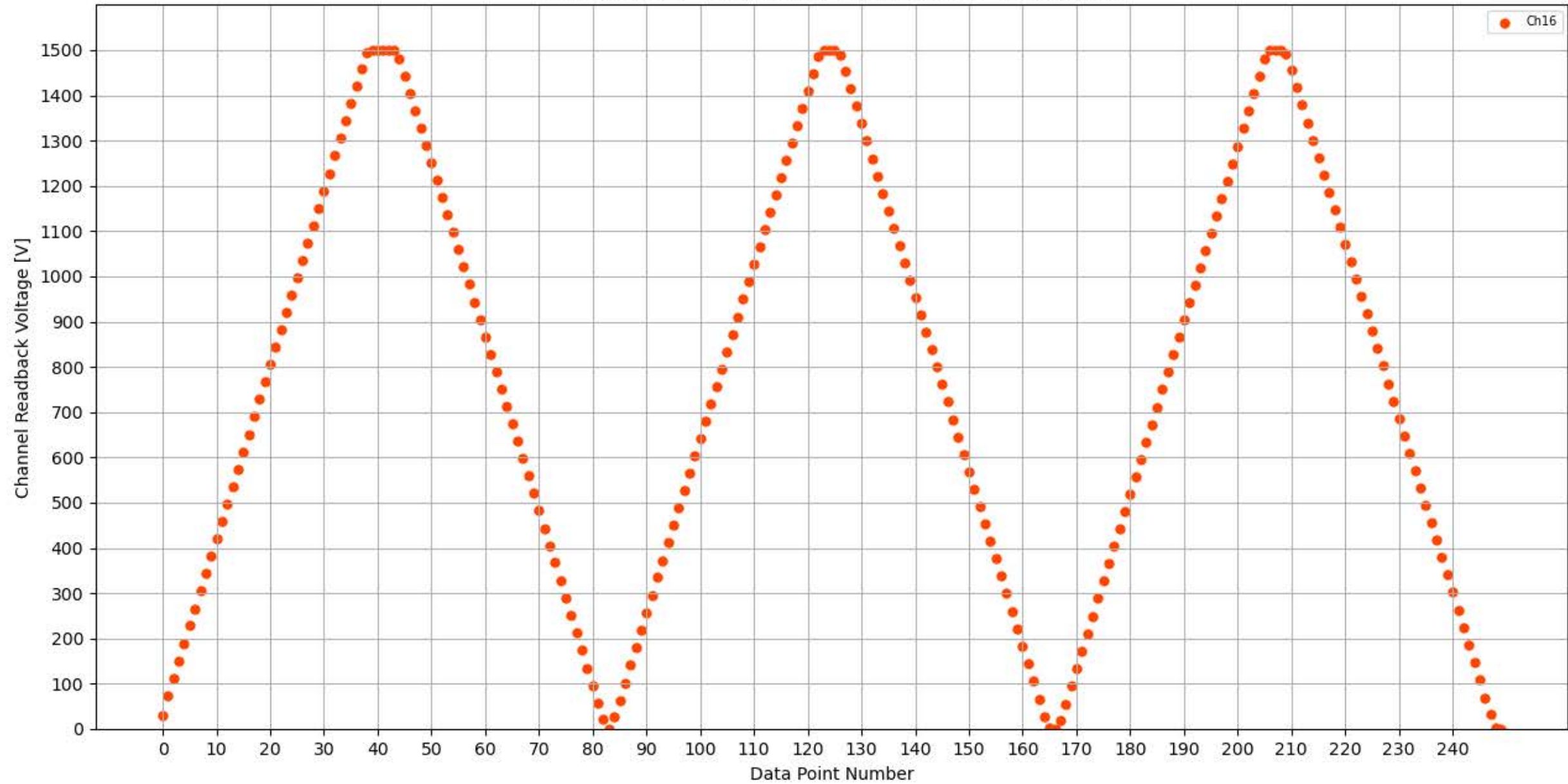
Voltage Ramp Test (Python) Bd #356, Slot #14, Ch #16
