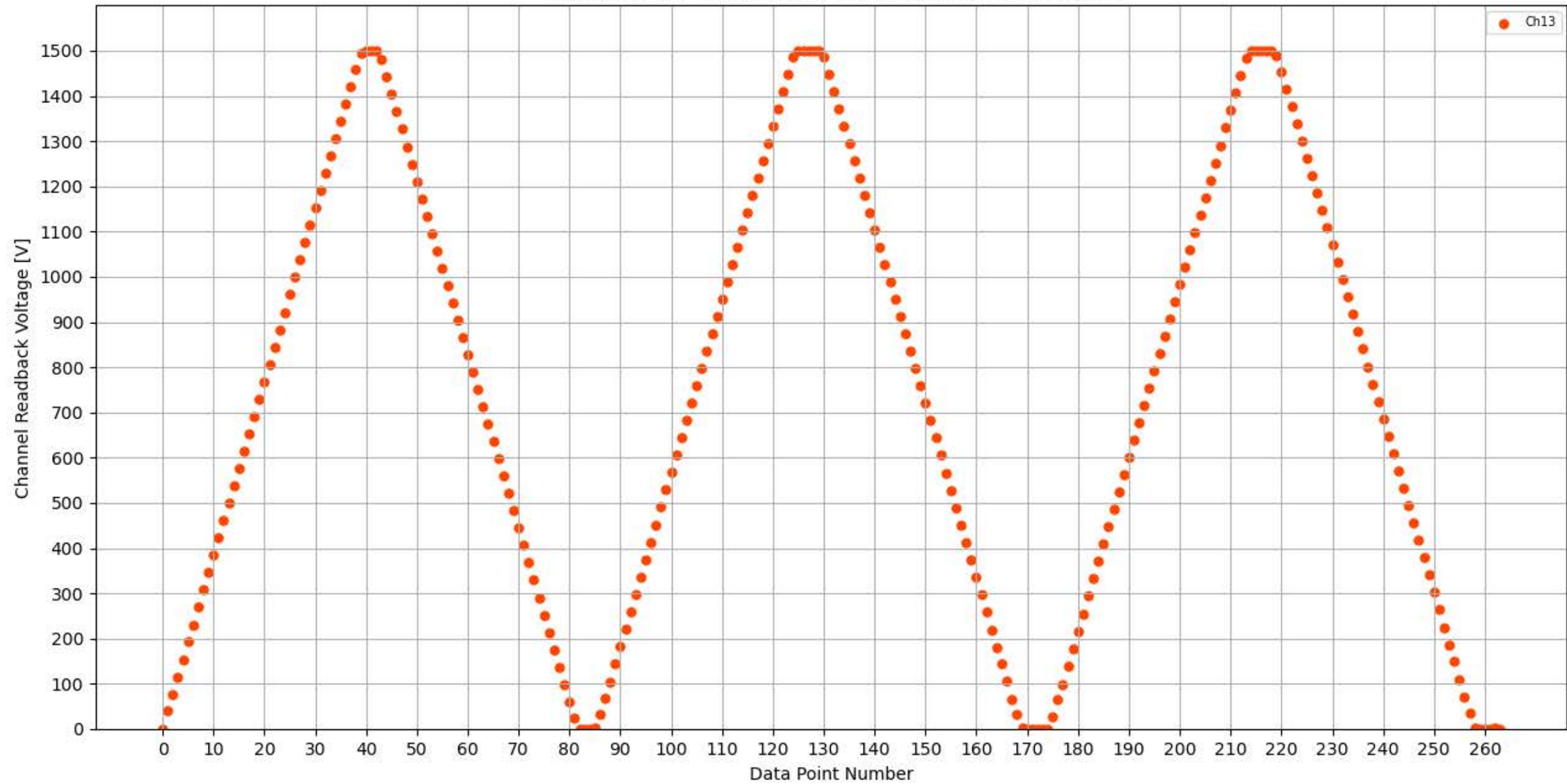
Voltage Ramp Test (Python) Bd #356, Slot #14, Ch #13
