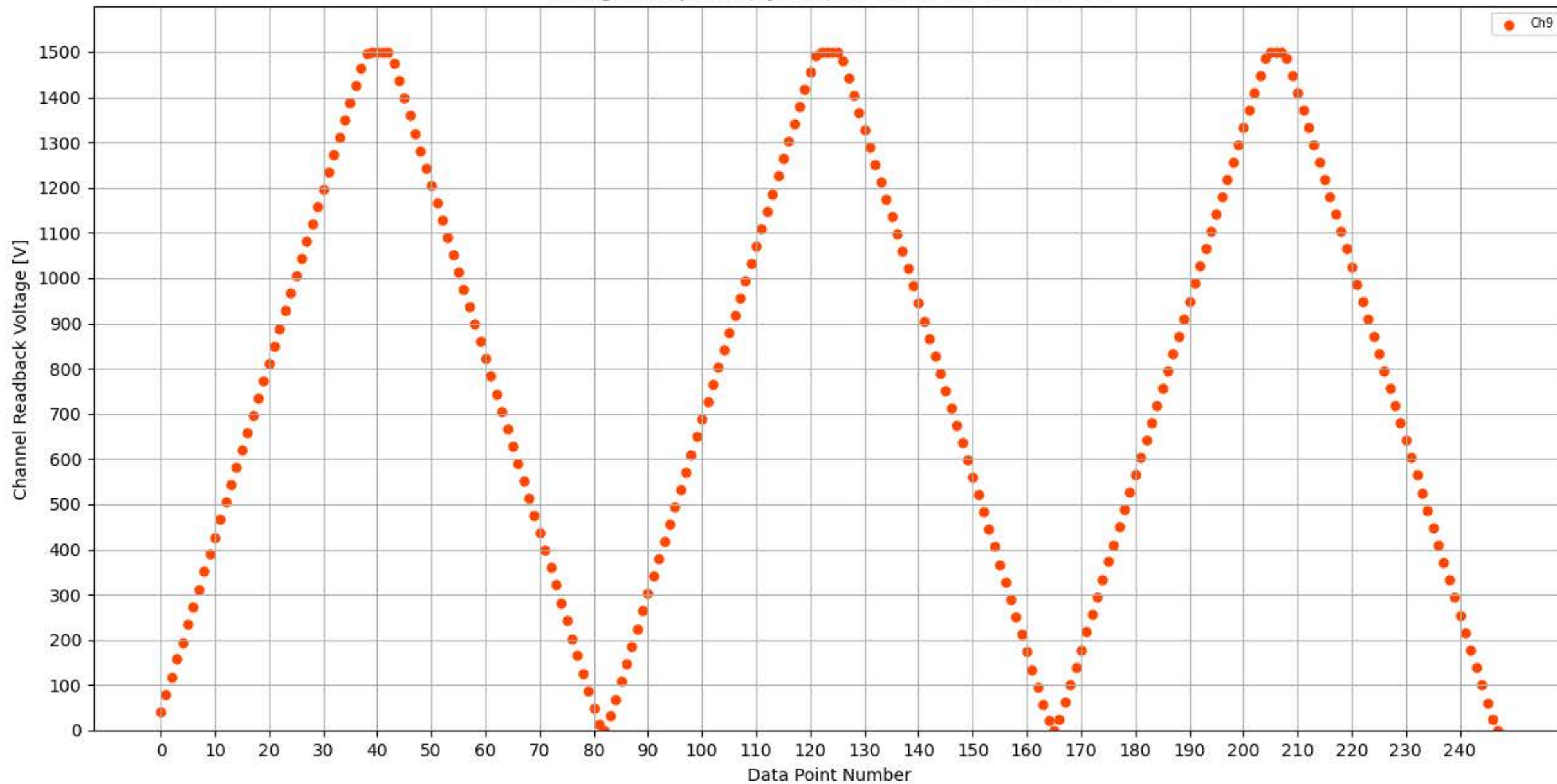
Voltage Ramp Test (Python) Bd #356, Slot #14, Ch #9
