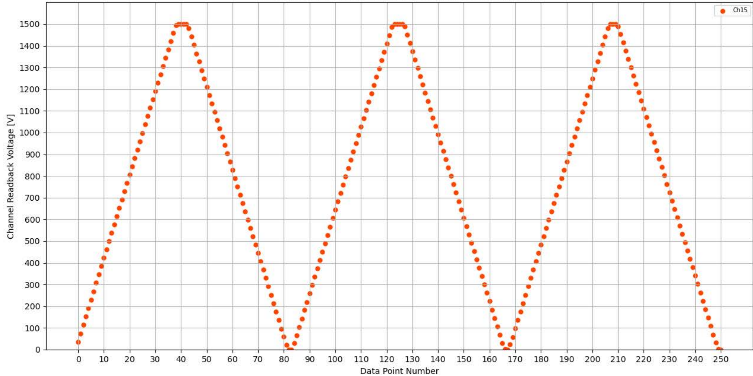
Voltage Ramp Test (Python) Bd #356, Slot #14, Ch #15
