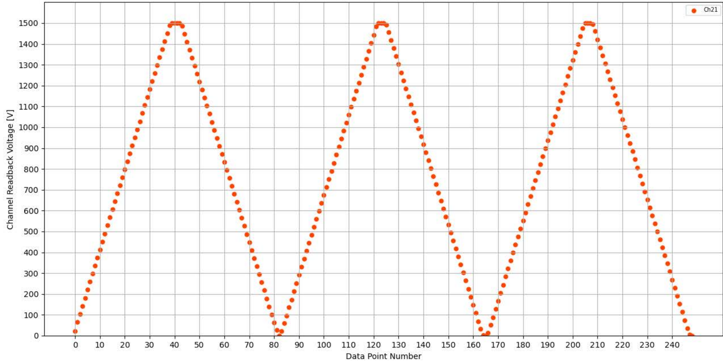
Voltage Ramp Test (Python) Bd #356, Slot #14, Ch #21
