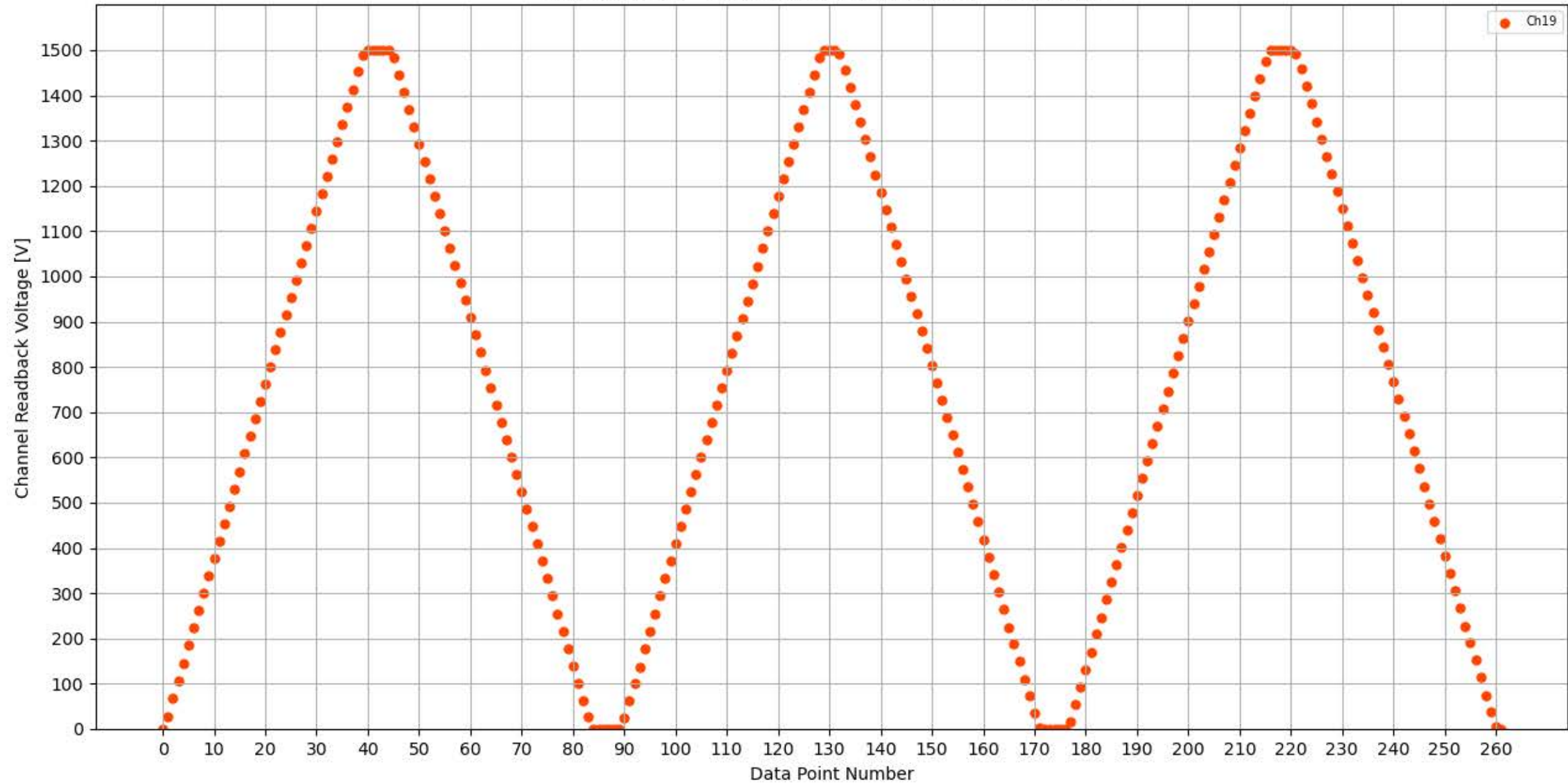
Voltage Ramp Test (Python) Bd #356, Slot #14, Ch #19
