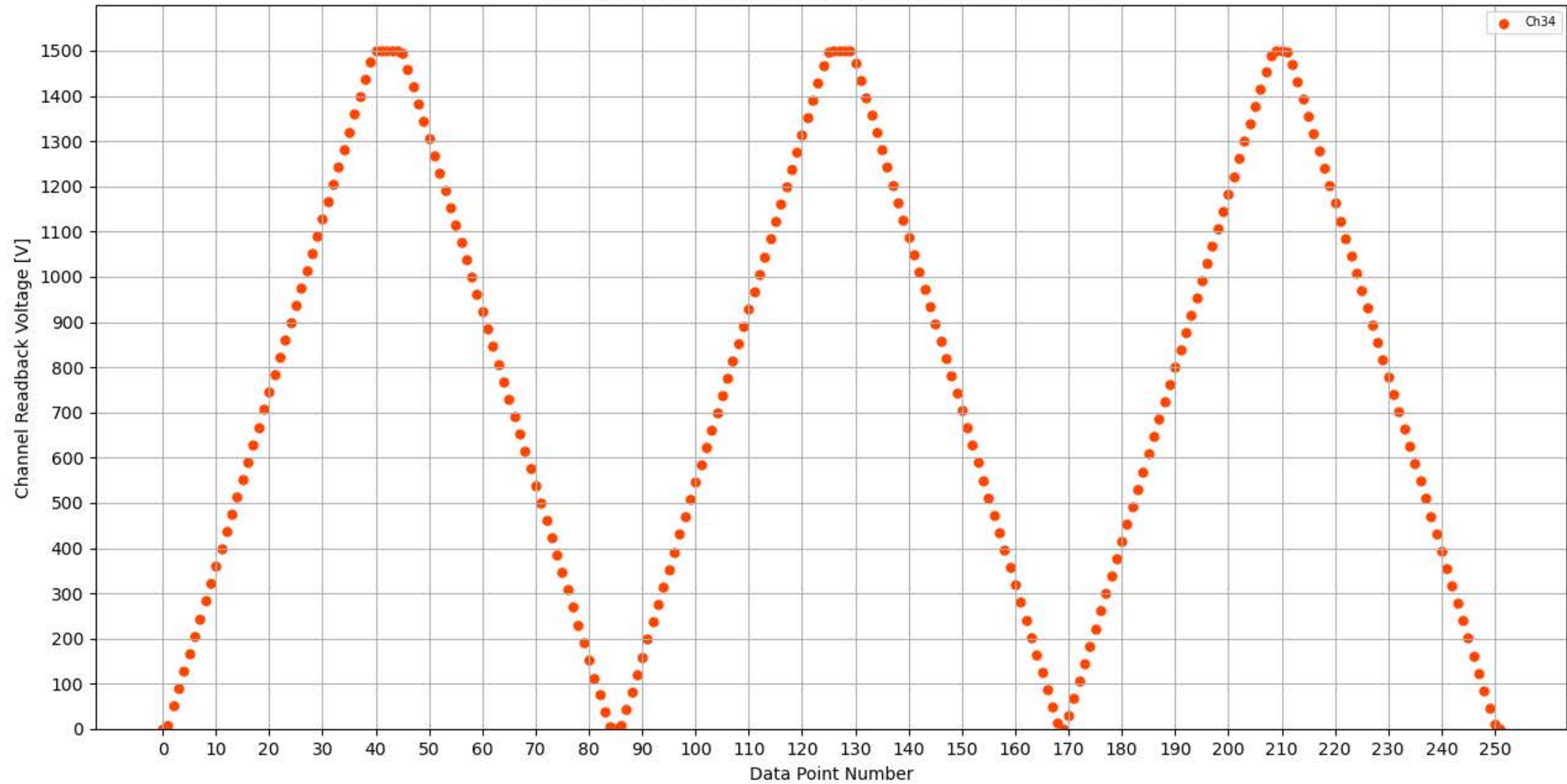
Voltage Ramp Test (Python) Bd #356, Slot #14, Ch #34
