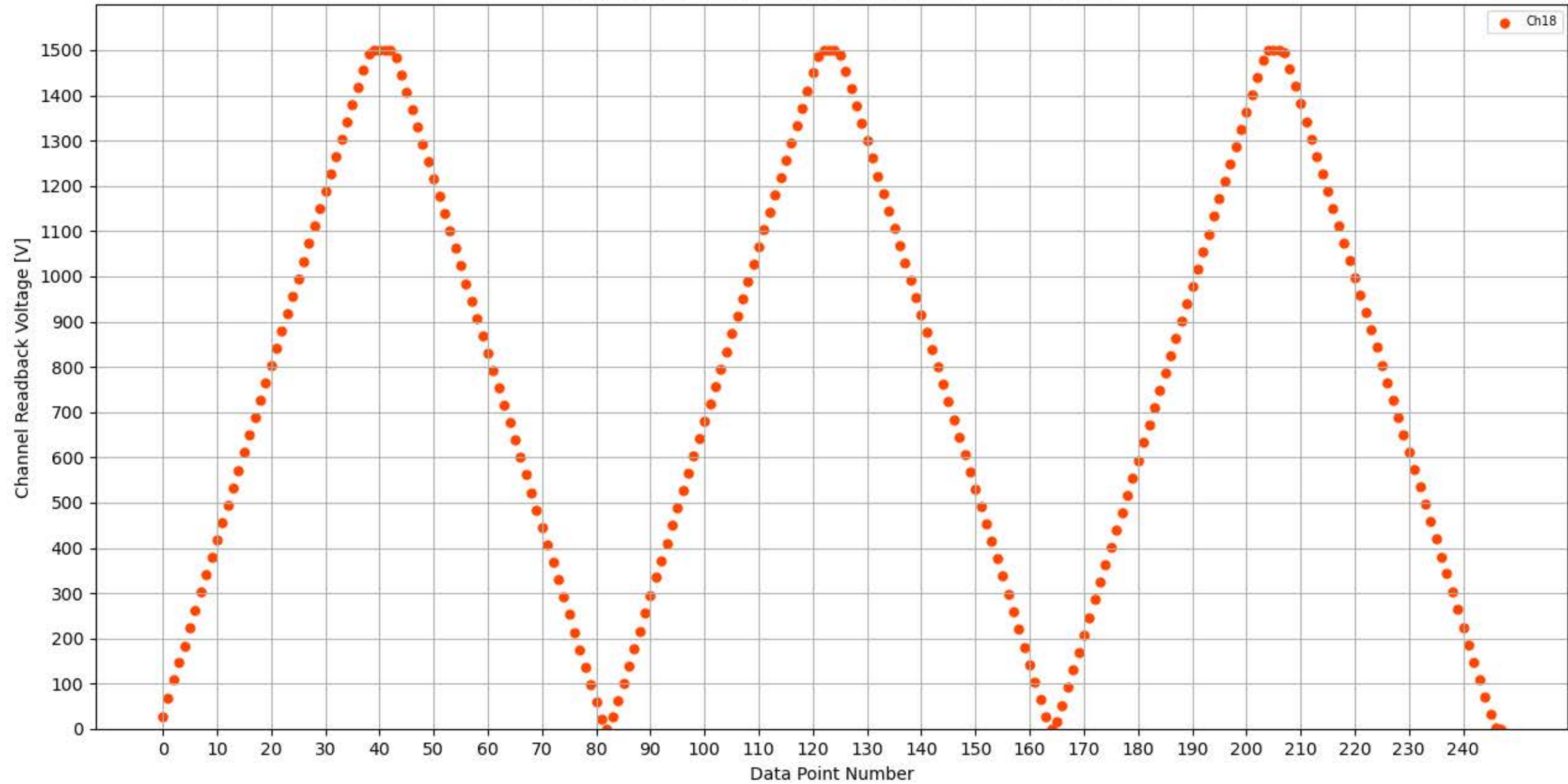
Voltage Ramp Test (Python) Bd #356, Slot #14, Ch #18
