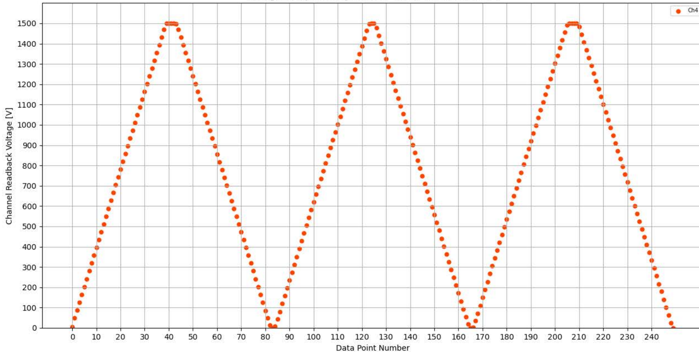
Voltage Ramp Test (Python) Bd #356, Slot #14, Ch #4
