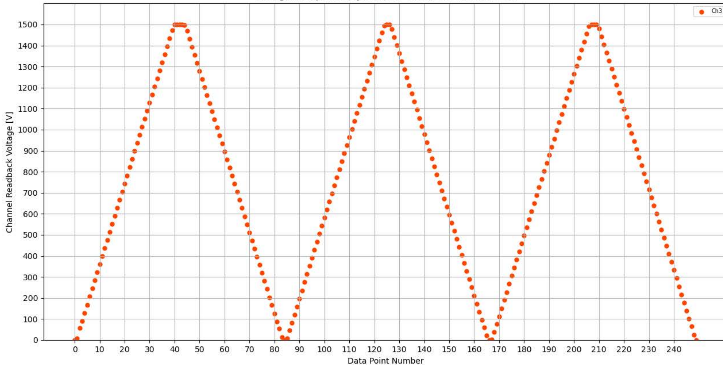
Voltage Ramp Test (Python) Bd #356, Slot #14, Ch #3
