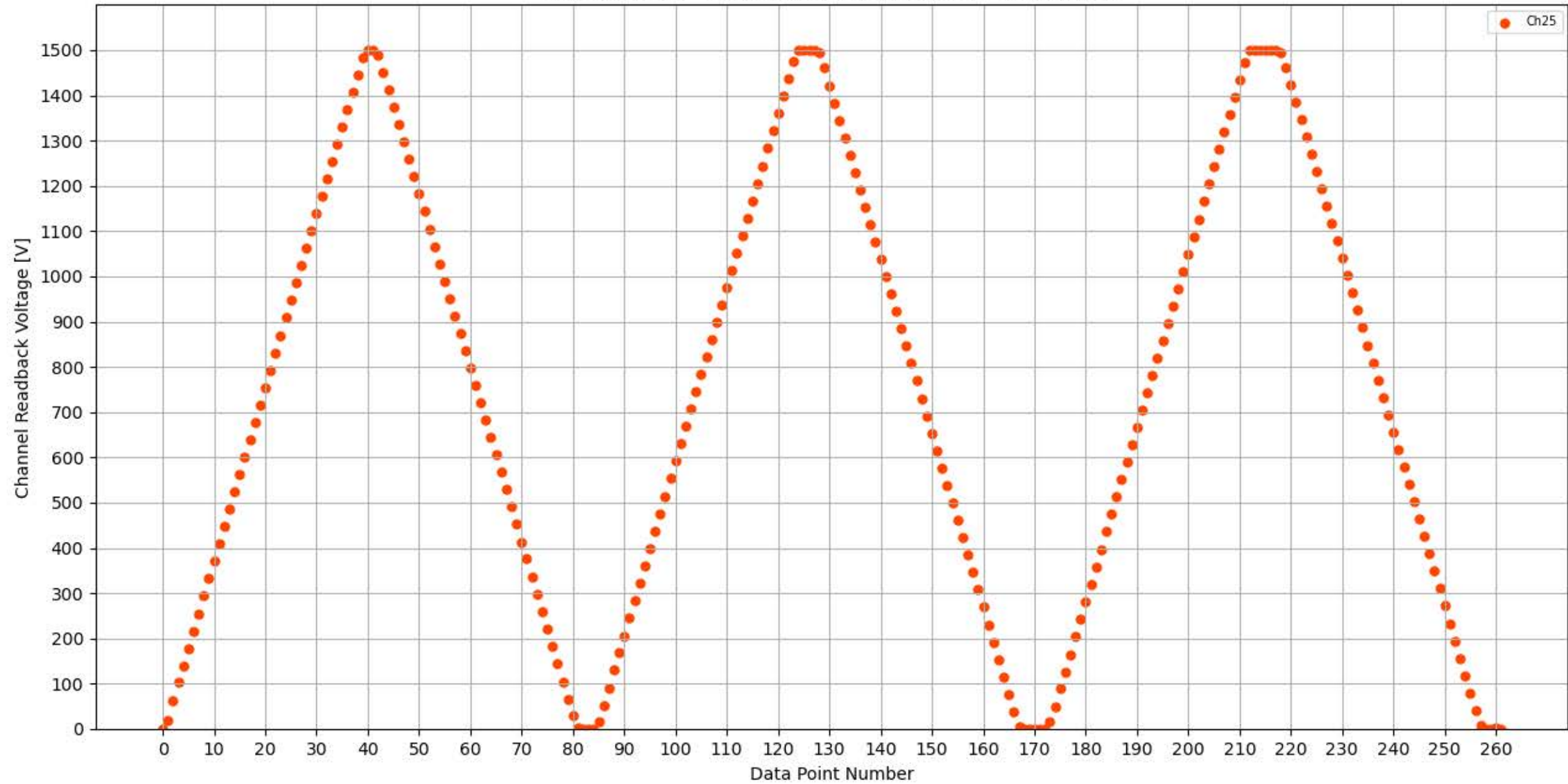
Voltage Ramp Test (Python) Bd #356, Slot #14, Ch #25
