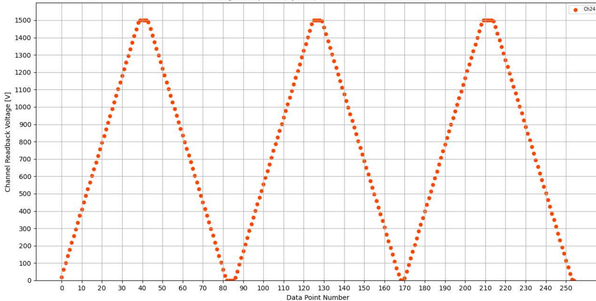
Voltage Ramp Test (Python) Bd #356, Slot #14, Ch #24
