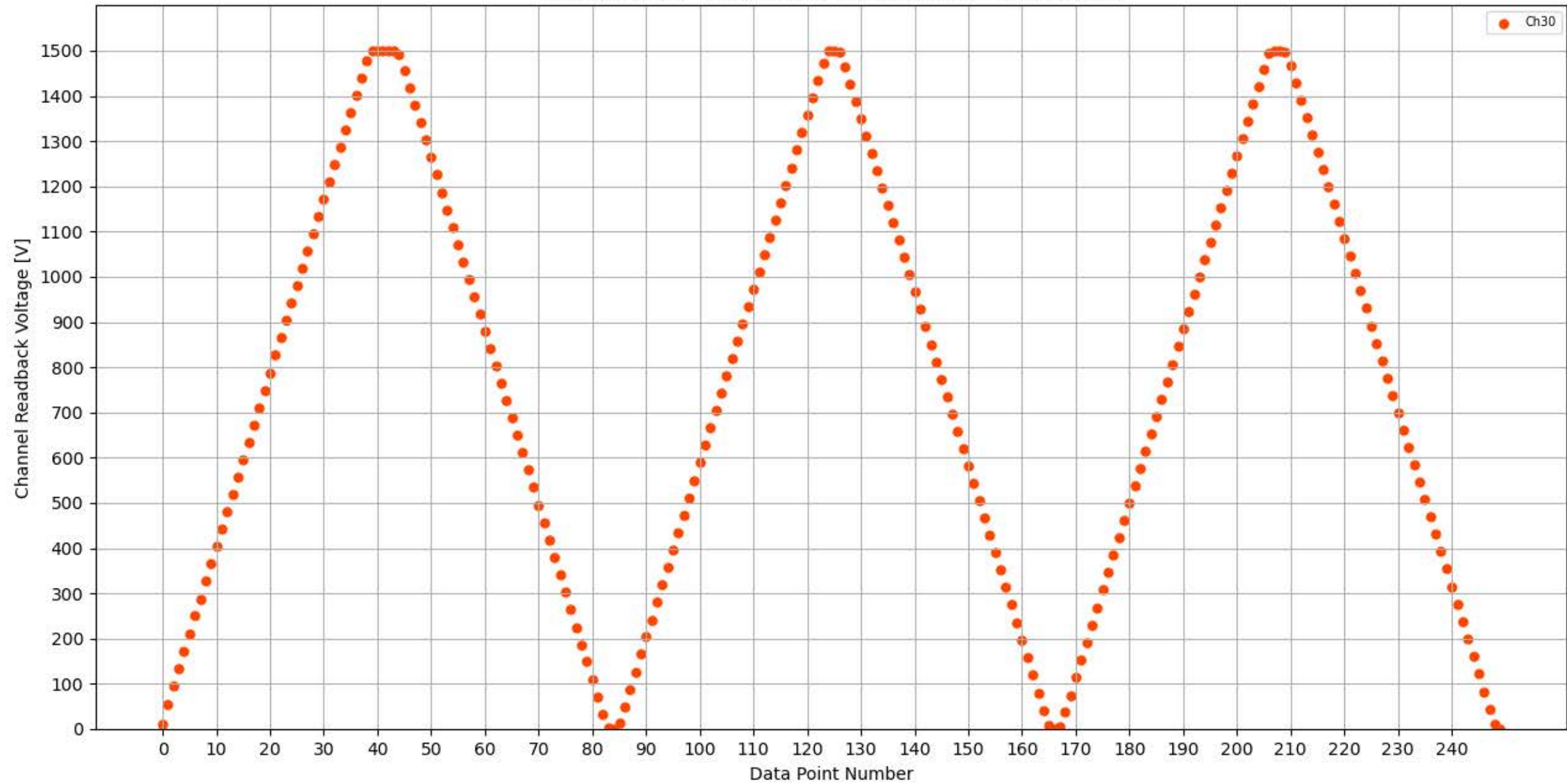
Voltage Ramp Test (Python) Bd #356, Slot #14, Ch #30
