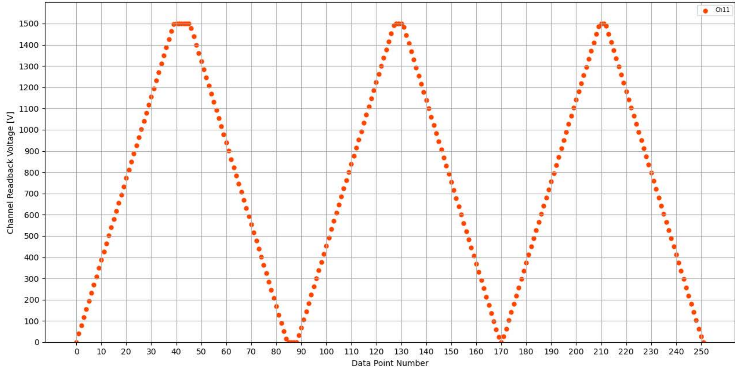
Voltage Ramp Test (Python) Bd #356, Slot #14, Ch #11
