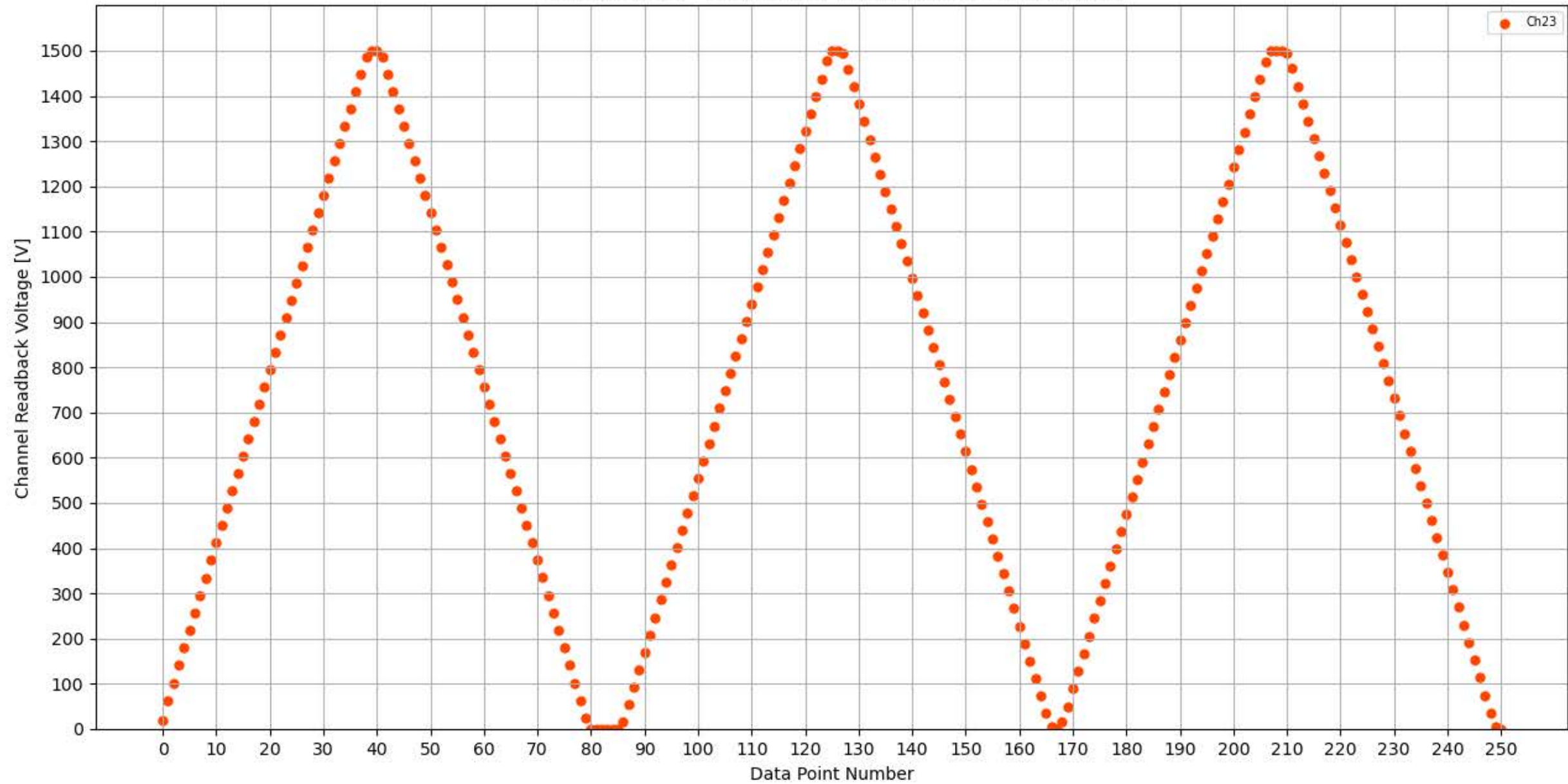
Voltage Ramp Test (Python) Bd #356, Slot #14, Ch #23
