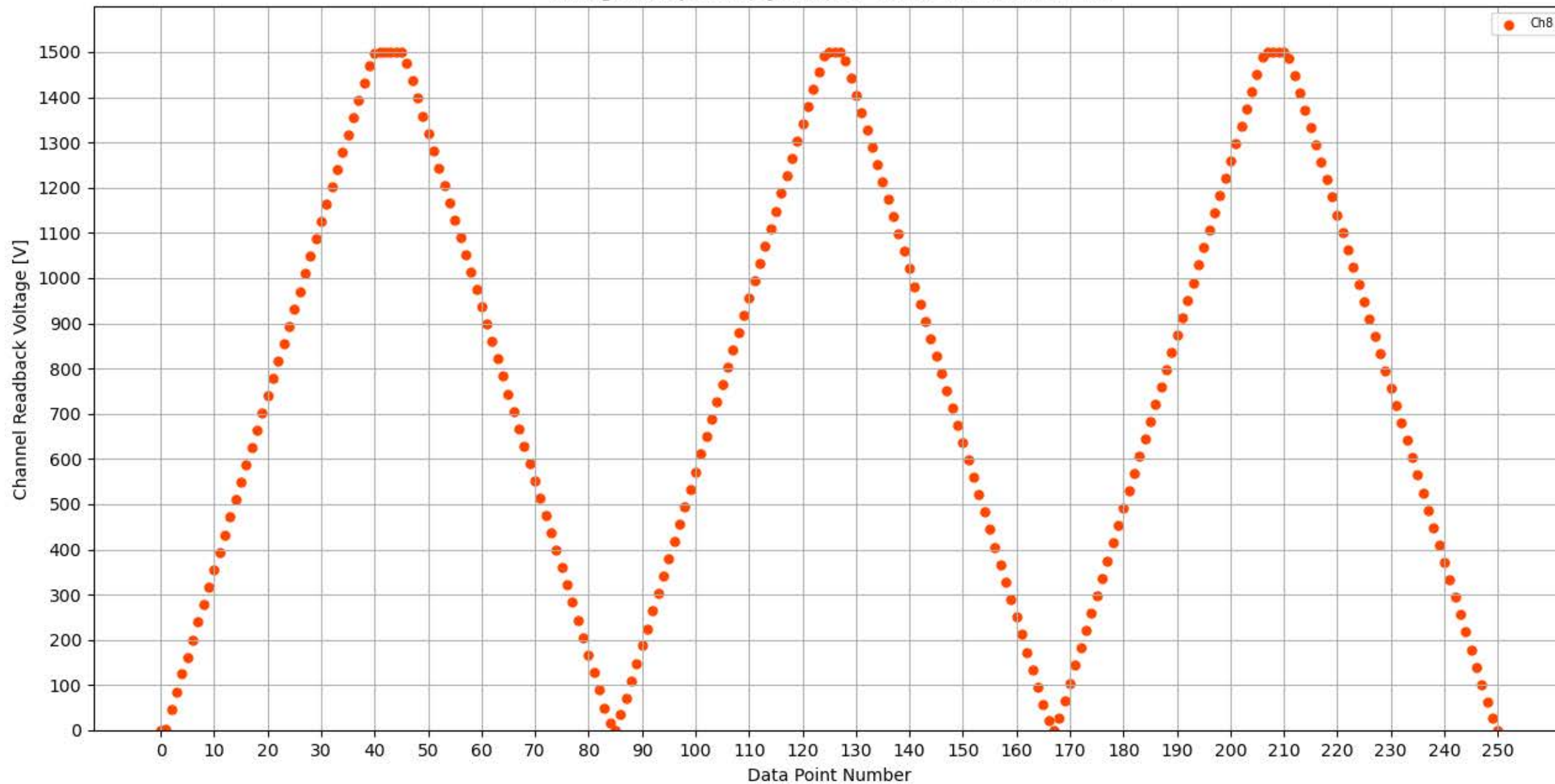
Voltage Ramp Test (Python) Bd #356, Slot #14, Ch #8
